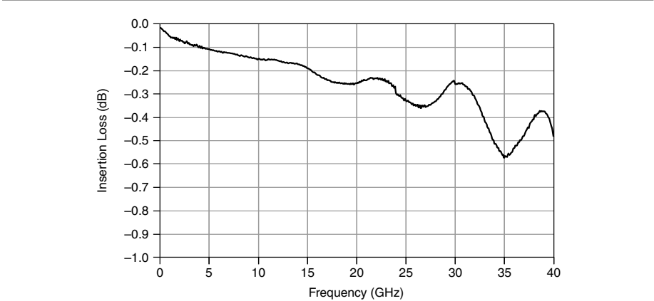
Figure 1. Typical Insertion Loss
