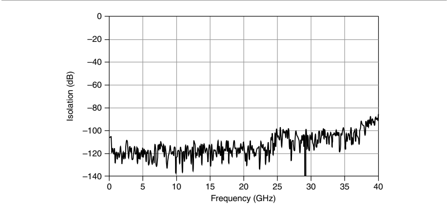
Figure 2. Typical Isolation
