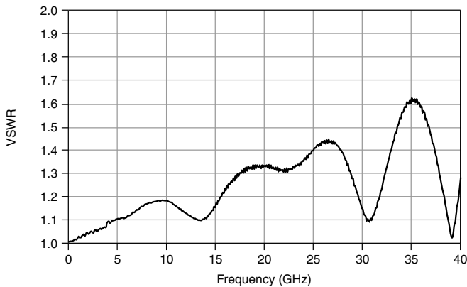
Figure 3. Typical VSWR
