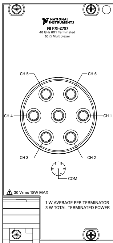
Figure 5. NI 2797 Front Panel
